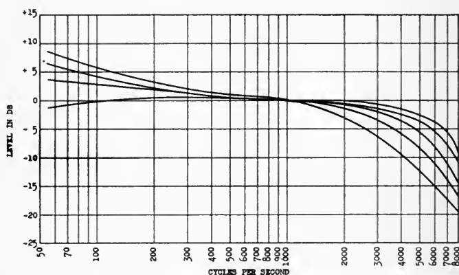
FIG. 5. Electrical characteristics of Simplex Type E system.
